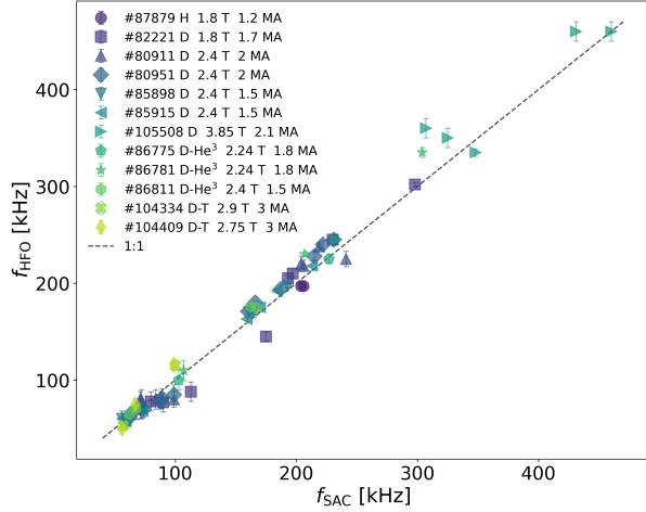
Figure 3: Measured n = 0 HFOs frequency versus the frequency of the correspondent n = 0 shear-Alfvén continuum minimum computed by CSMISH.
